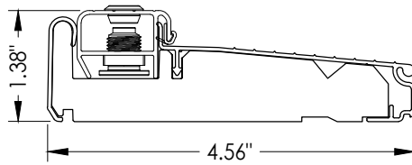
4 INSWING ADJUSTABLE THRESHOLD ZAI4565FN MAX. DESIGN PRESSURE = \pm 50 PSF
