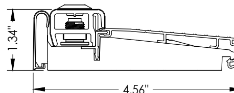
5 INSWING ADJUSTABLE THRESHOLD ZAI4565RDS MAX. DESIGN PRESSURE = \pm 45 PSF
