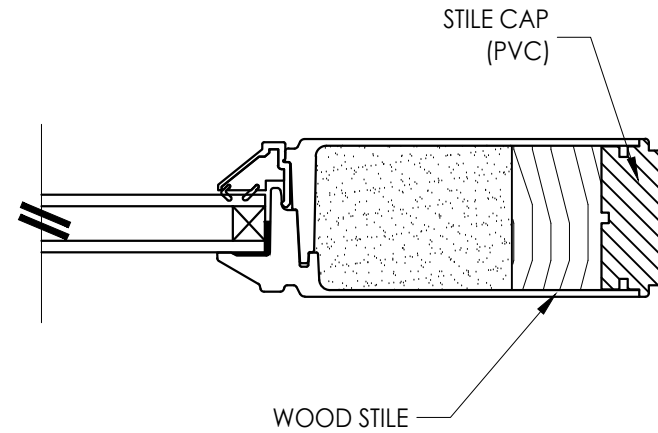
1 3 HORIZONTAL CROSS SECTION
