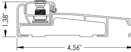
3 INSWING ADJUSTABLE THRESHOLD ZAILAA4565 MAX. DESIGN PRESSURE = \pm 50 PSF
